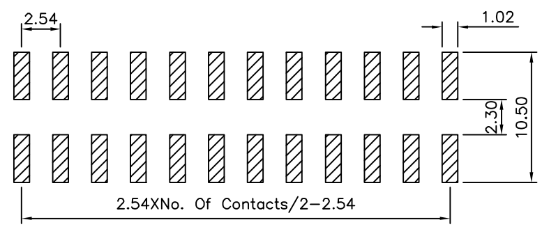
△ Recommended P.C.B. Layout PCB Tolerance:±0.05 (Top View)
